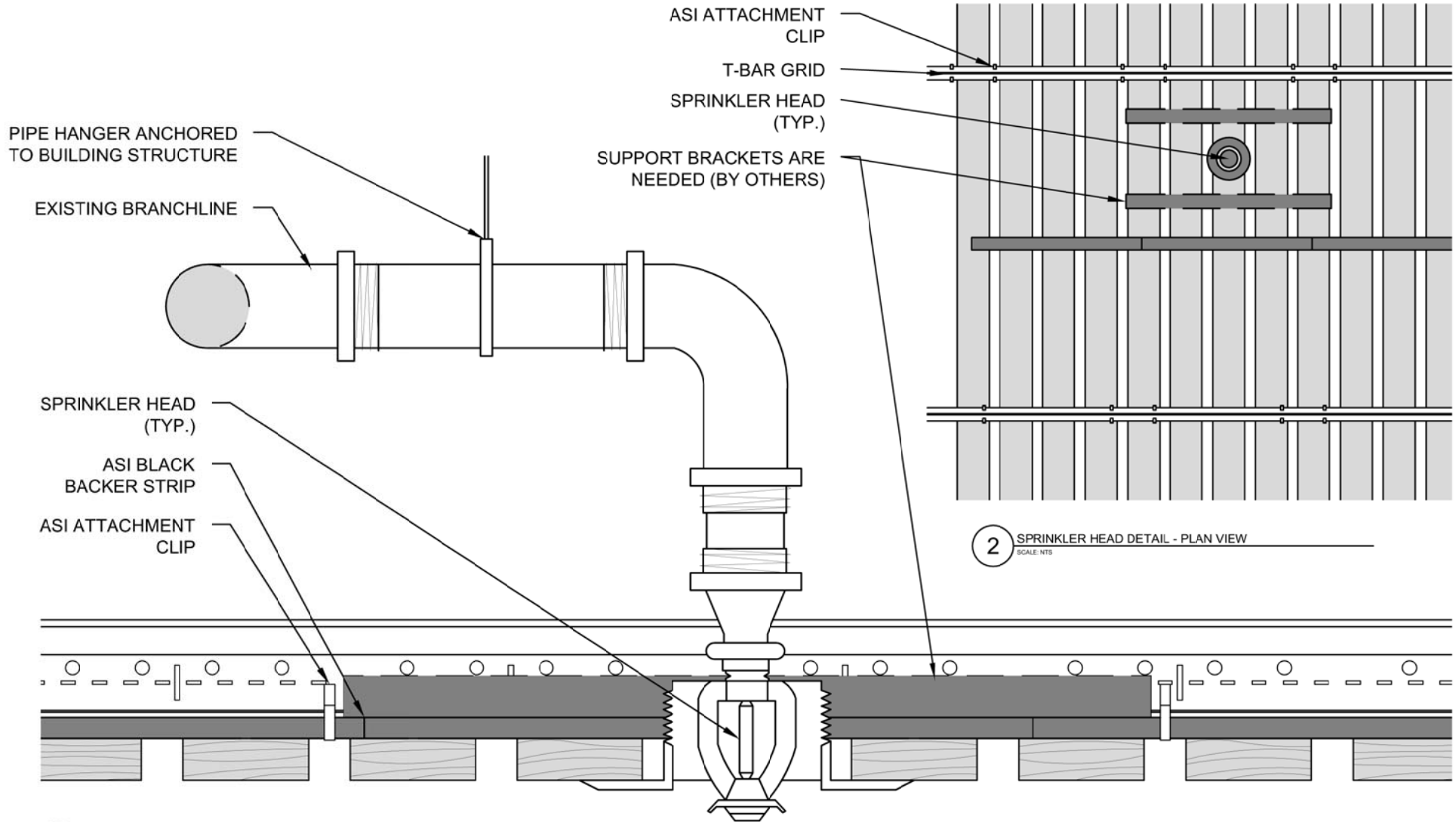
1 SPRINKLER HEAD DETAIL - SECTION VIEW SCALE: NTS
