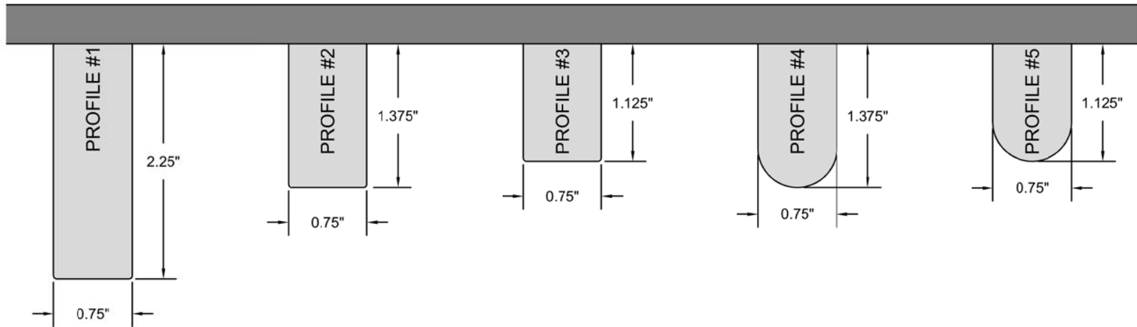
1 COMMON STAVE PROFILES SCALE: NTS
