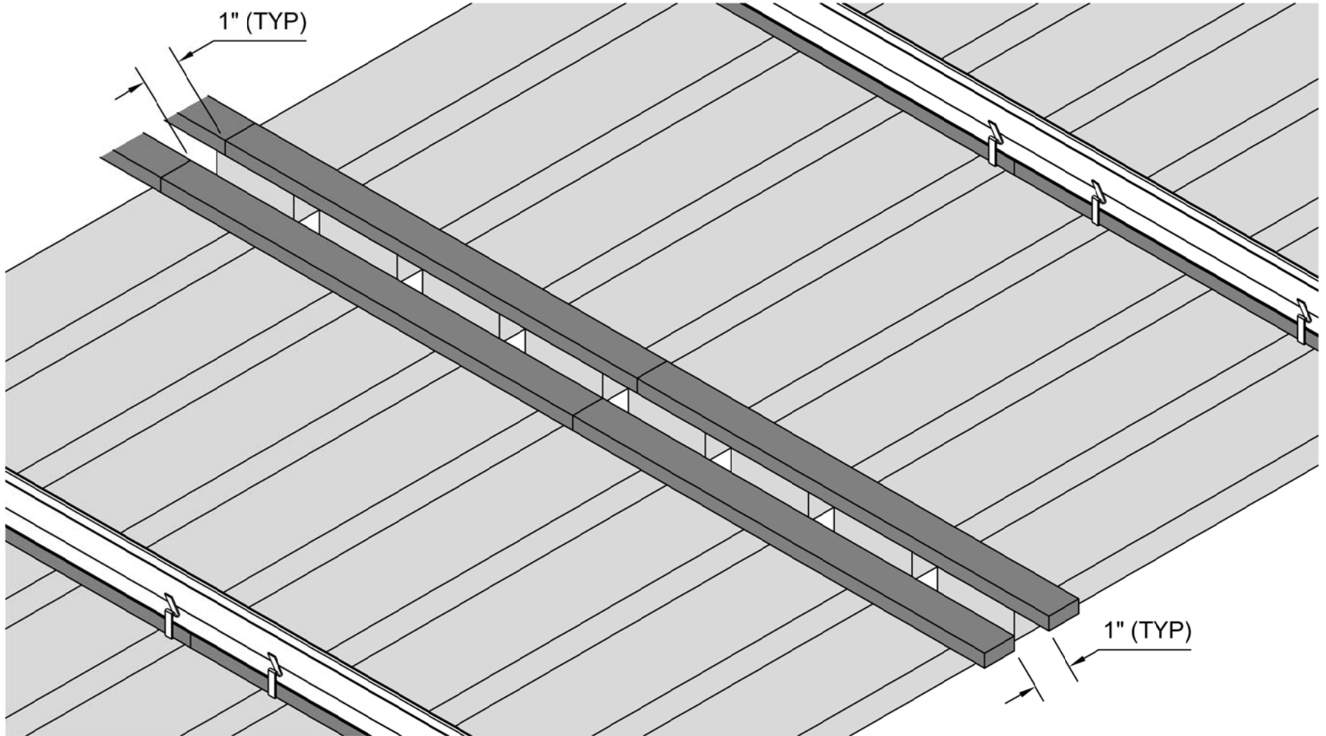
1 GRILLE ALIGNMENT (TYP) SCALE: NTS
