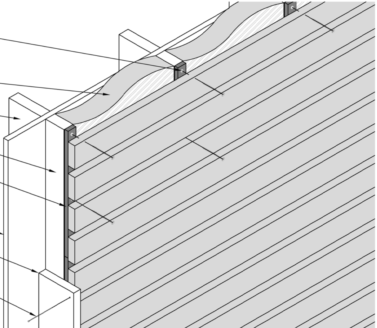
1 DIRECT ATTACHMENT (TYP) SCALE: NTS
