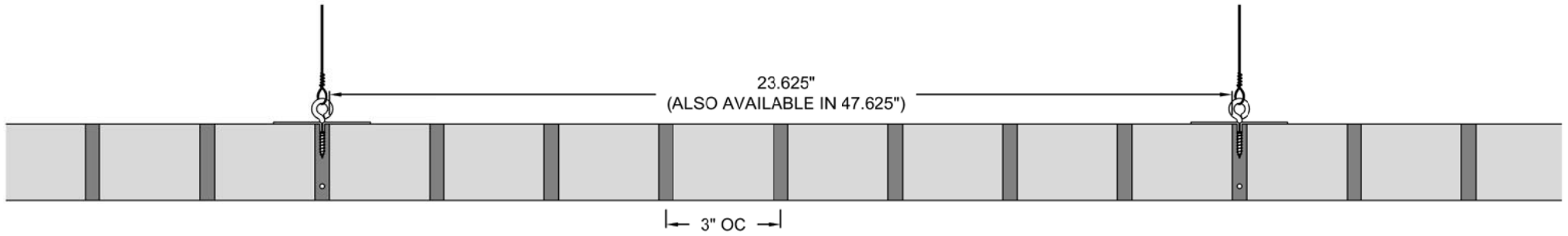
1 SECTION DETAIL - 3" OC ACTUAL DIMENSIONS SCALE: NTS
