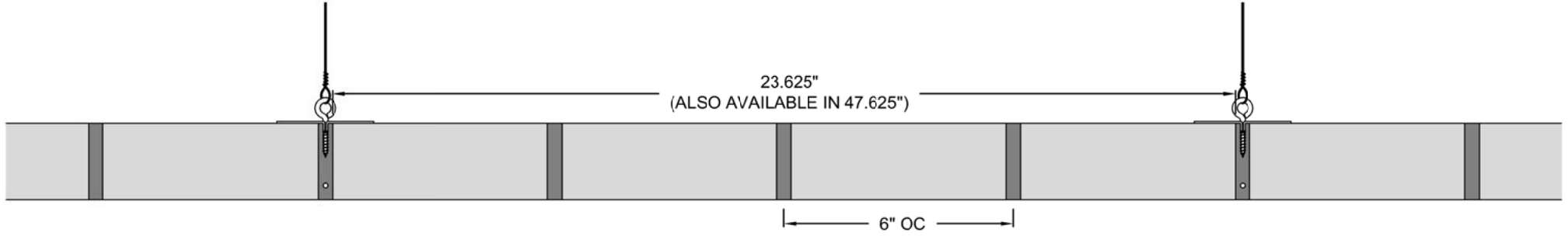
3 SECTION DETAIL - 6" OC ACTUAL DIMENSIONS SCALE: NTS
