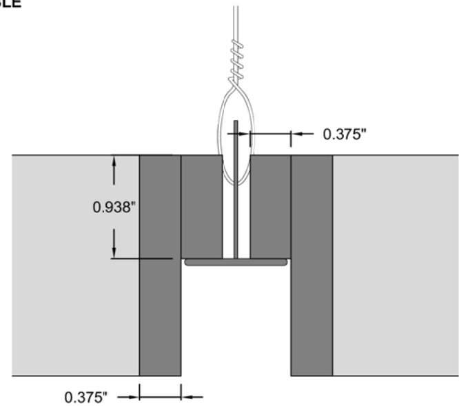
2 T-GRID ATTACHMENT DETAIL SCALE: NTS
