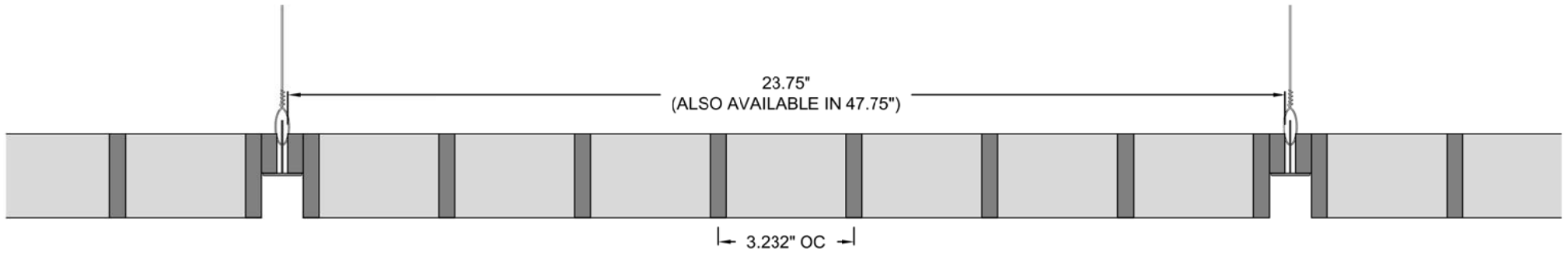
1 SECTION DETAIL - 3" OC ACTUAL DIMENSIONS SCALE: NTS
