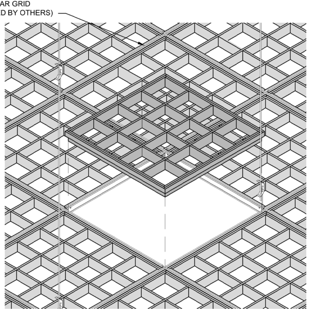
2 ISOMETRIC VIEW (TYP.) SCALE: NTS
