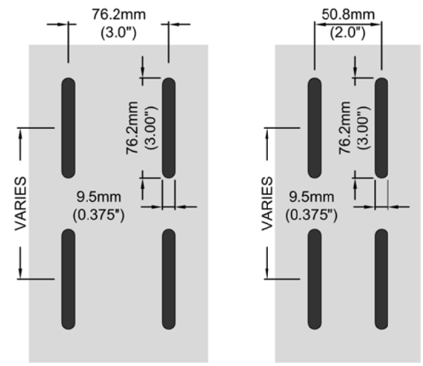
2 STANDARD SLOTTED PERFORATION TYPES SCALE: NTS
