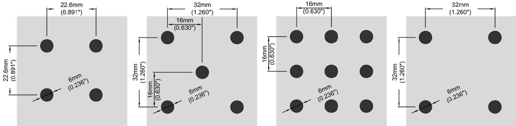
1 STANDARD CIRCULAR PERFORATION TYPES (PERFORATION = 6mm/0.236") SCALE: NTS
