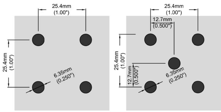
1 STANDARD CIRCULAR PERFORATION TYPES (CONT.) PERFORATION = 6.35mm/0.25" SCALE: NTS
