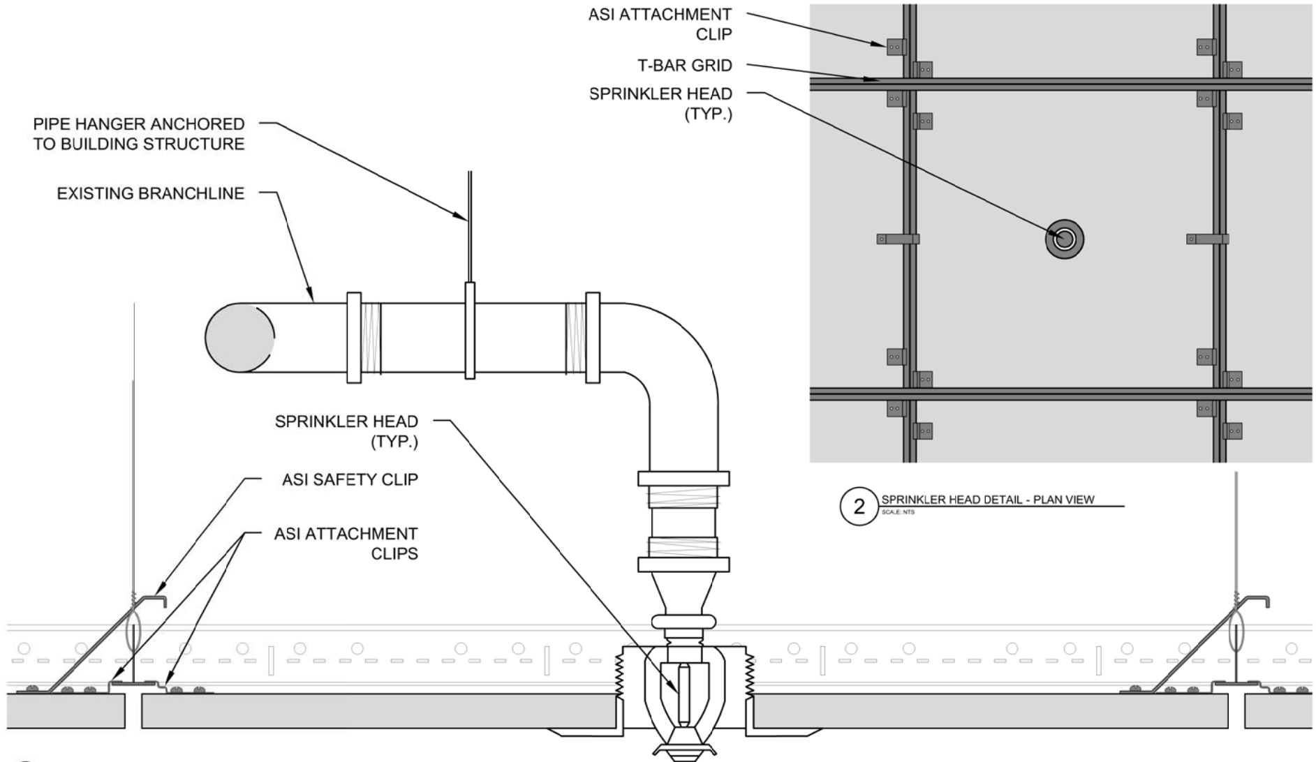
1 SPRINKLER HEAD DETAIL - SECTION VIEW SCALE: NTS
