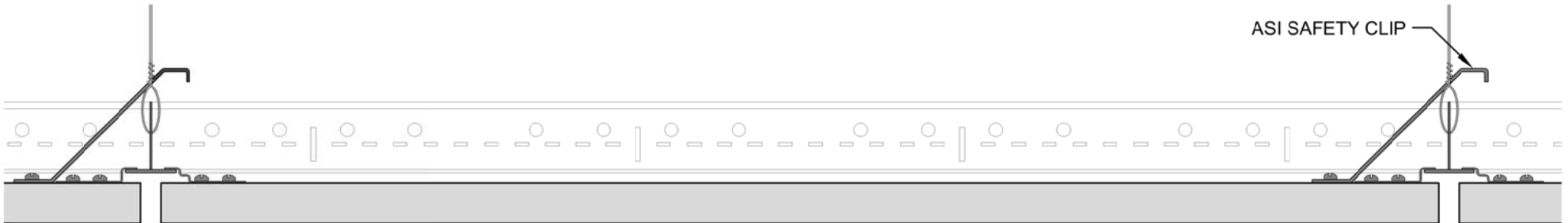
3 SECTION DETAIL - \frac{3}{8} " REVEAL SCALE: NTS
