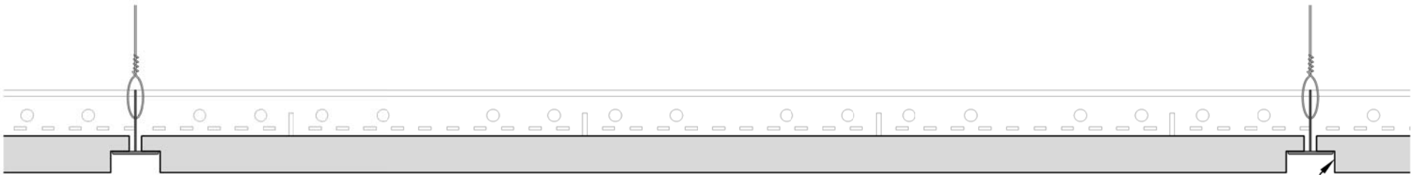
2 SECTION DETAIL - 1" TEGULAR REVEAL (ALSO AVAILABLE WITH \frac{5}{8} " REVEAL) SCALE: NTS
