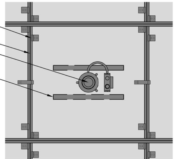
2 RECESSED LIGHT DETAIL - PLAN VIEW SCALE: NTS
