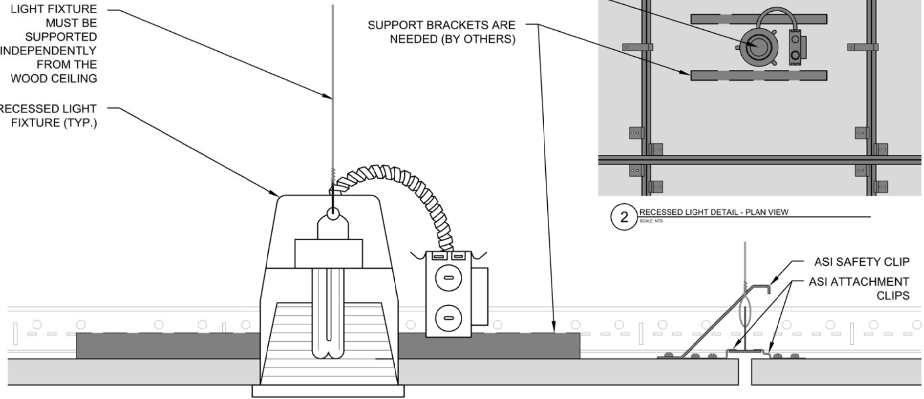
1 RECESSED LIGHT DETAIL - SECTION VIEW SCALE: NTS
