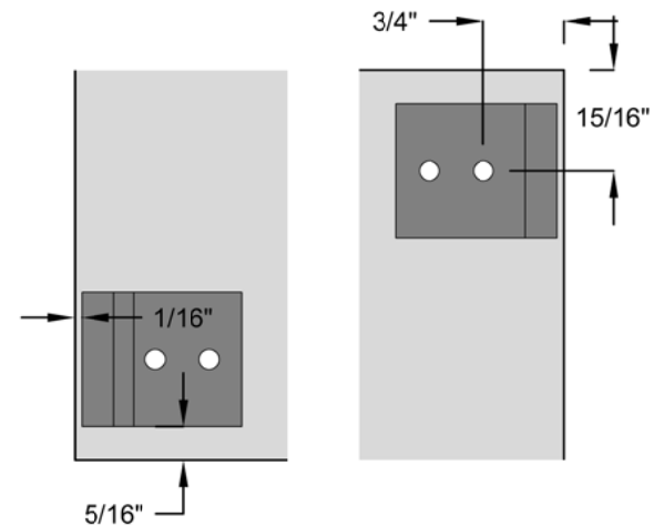
3 CLIP PLACEMENT - CLIP 'B' & CLIP 'D' SCALE: NTS
