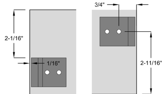
2 CLIP PLACEMENT - CLIP 'A' & CLIP 'C' SCALE: NTS
