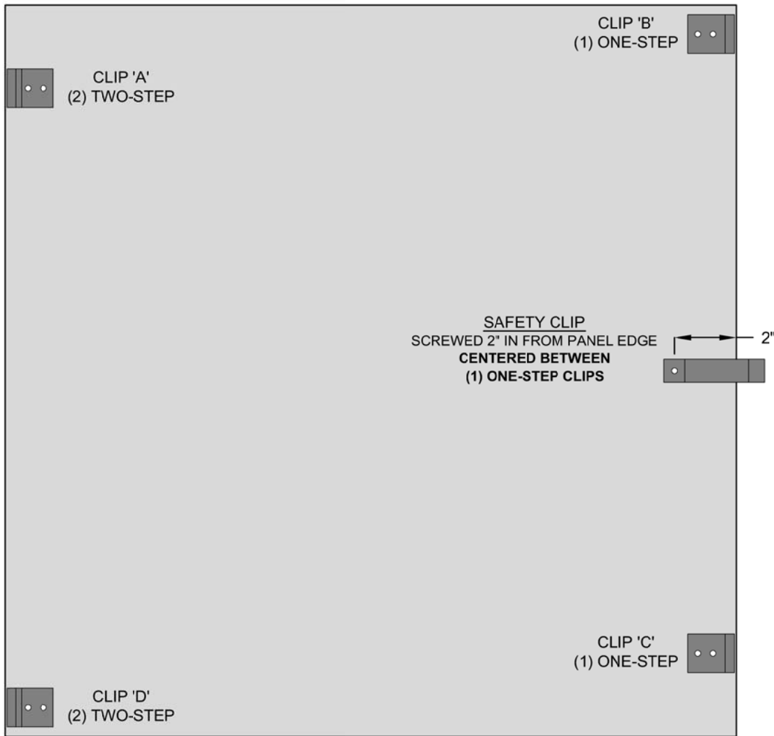
1 CLIP PLACEMENT - \frac{3}{8} " REVEAL PANEL SCALE: NTS
