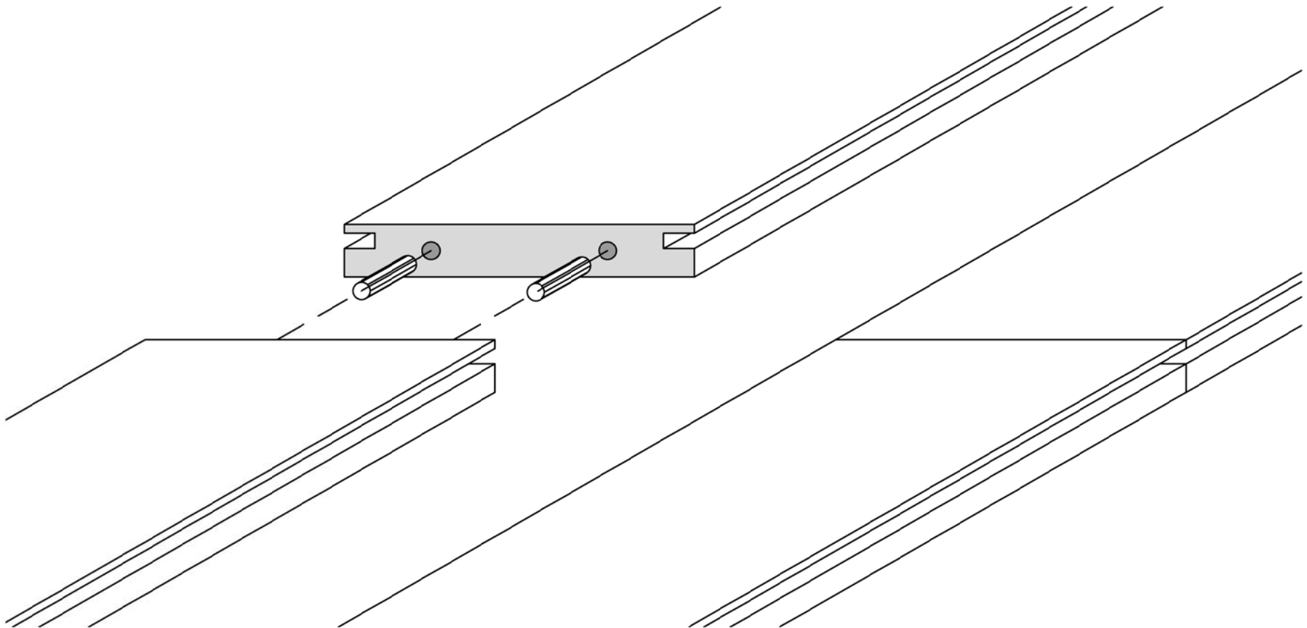
1 DOWEL ALIGNMENT SCALE: NTS
