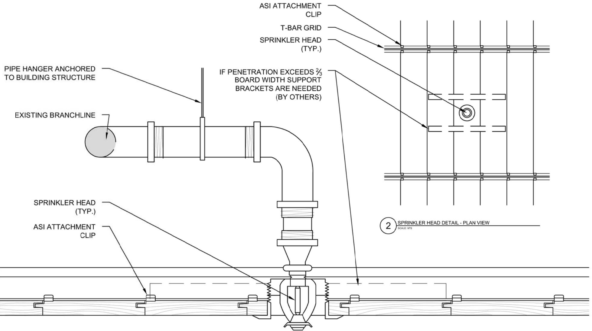
1 SPRINKLER HEAD DETAIL - SECTION VIEW SCALE: NTS
