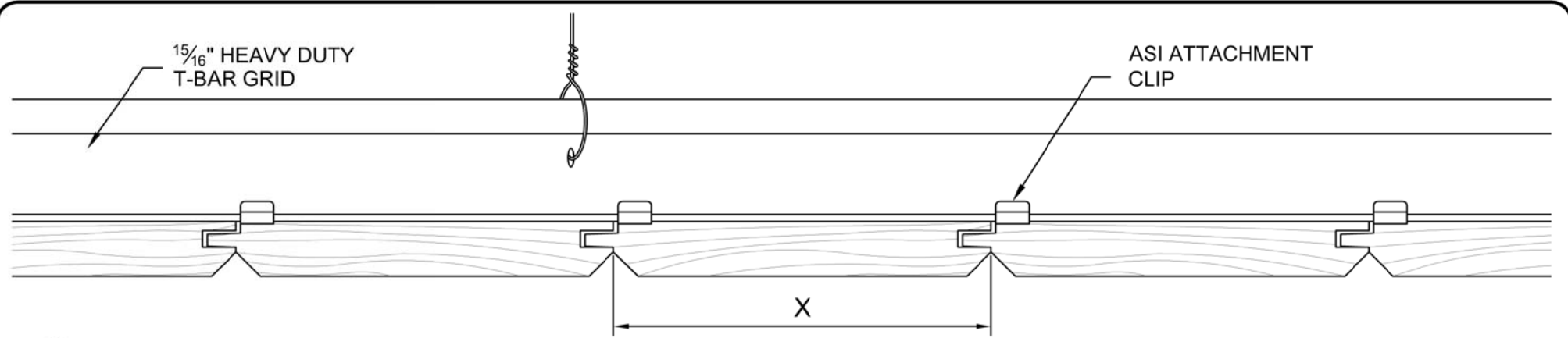
1 SECTION DETAIL SCALE: NTS
