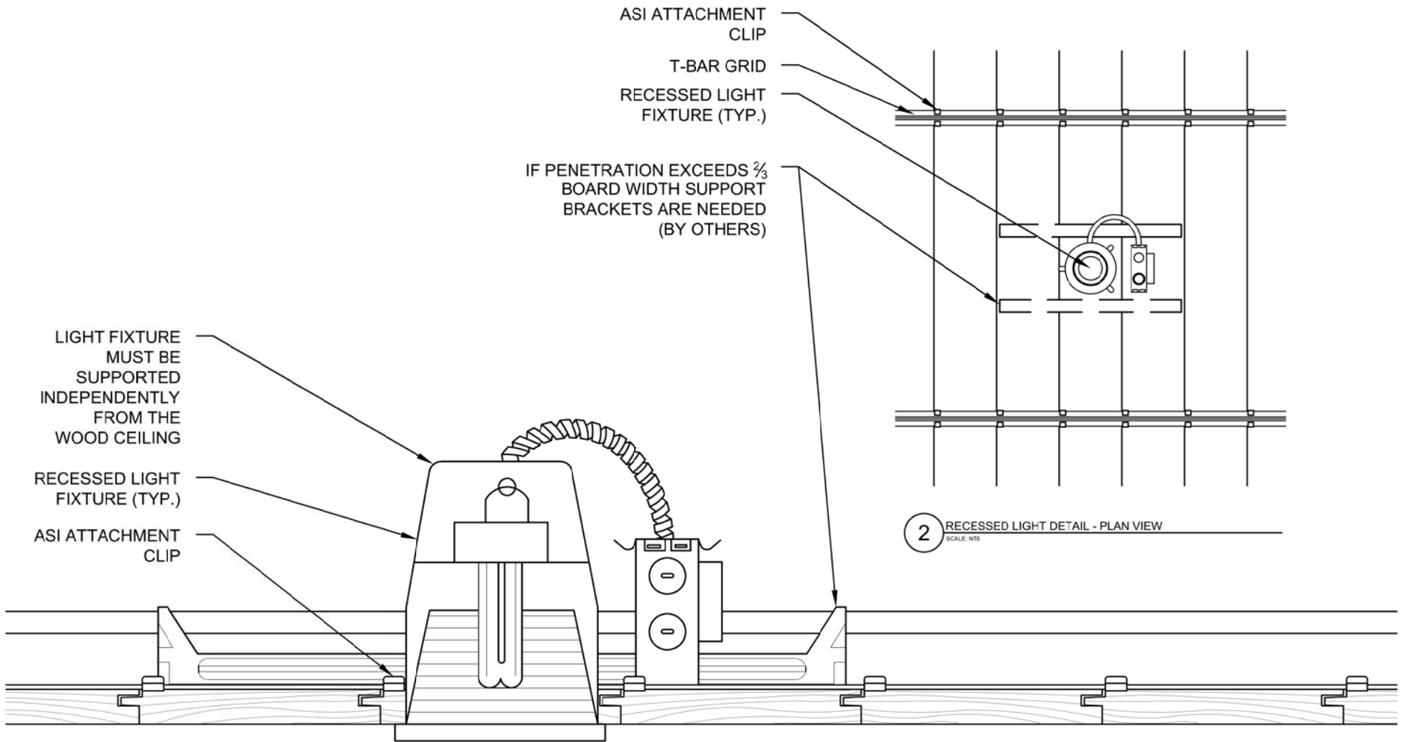
1 RECESSED LIGHT DETAIL - SECTION VIEW SCALE: NTS
