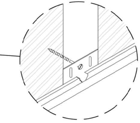
2 DIRECT ATTACHMENT - ENLARGED DETAIL SCALE: NTS
