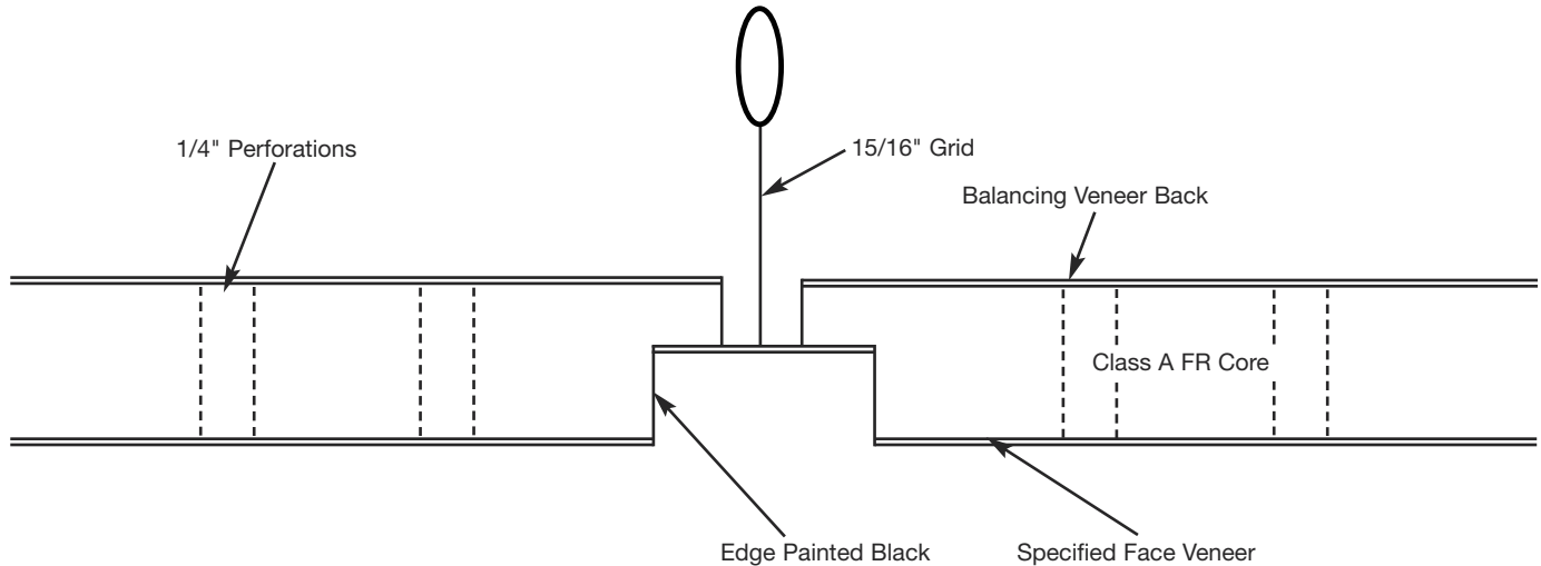
Standard Edge Detail (15/16" Grid)
