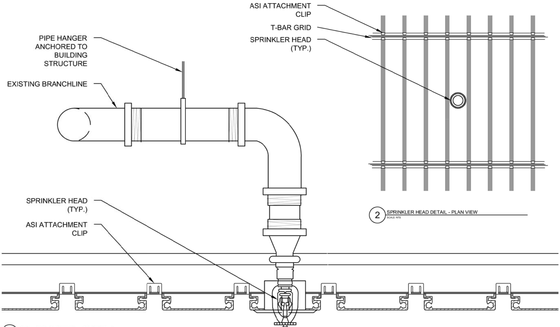
1 SPRINKLER HEAD DEATIL - SECTION VIEW SCALE: NTS
