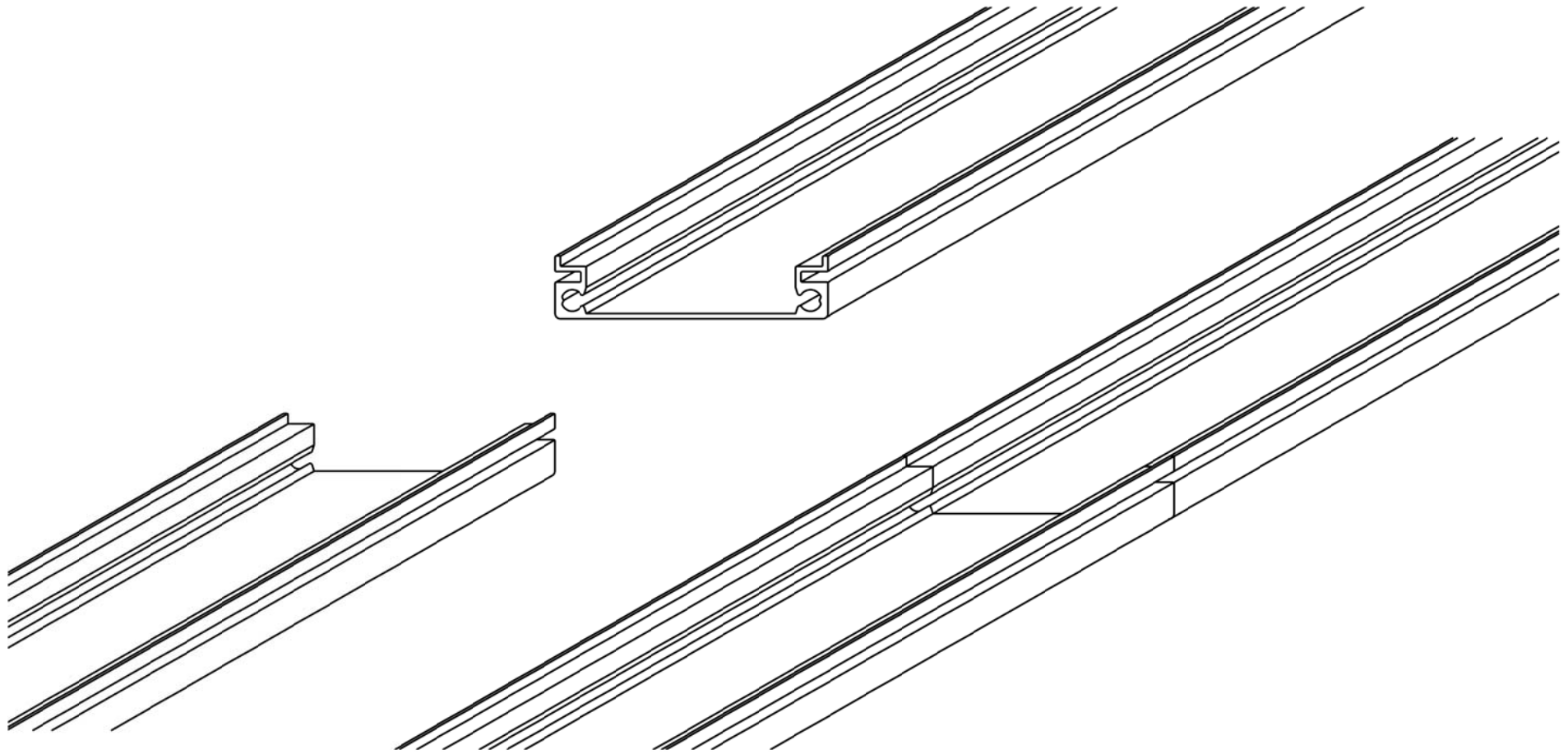
1 SPLINE ALIGNMENT SCALE: NTS
