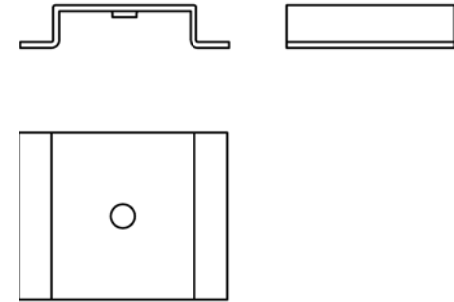
3 DIRECT ATTACHMENT CLIP SCALE: NTS
