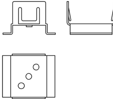
2 T-GRID SUSPENDED ATTACHMENT CLIP SCALE: NTS
