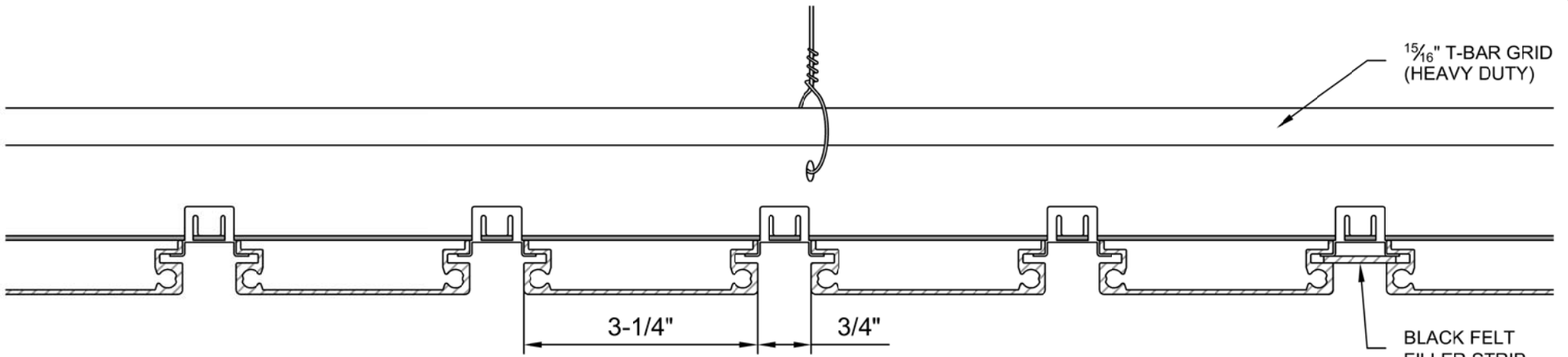
1 SECTION DETAIL SCALE: NTS
