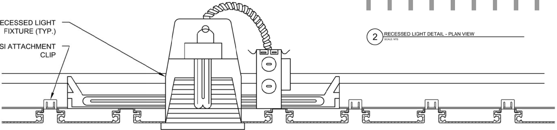
1 RECESSED LIGHT DETAIL - SECTION VIEW SCALE: NTS
