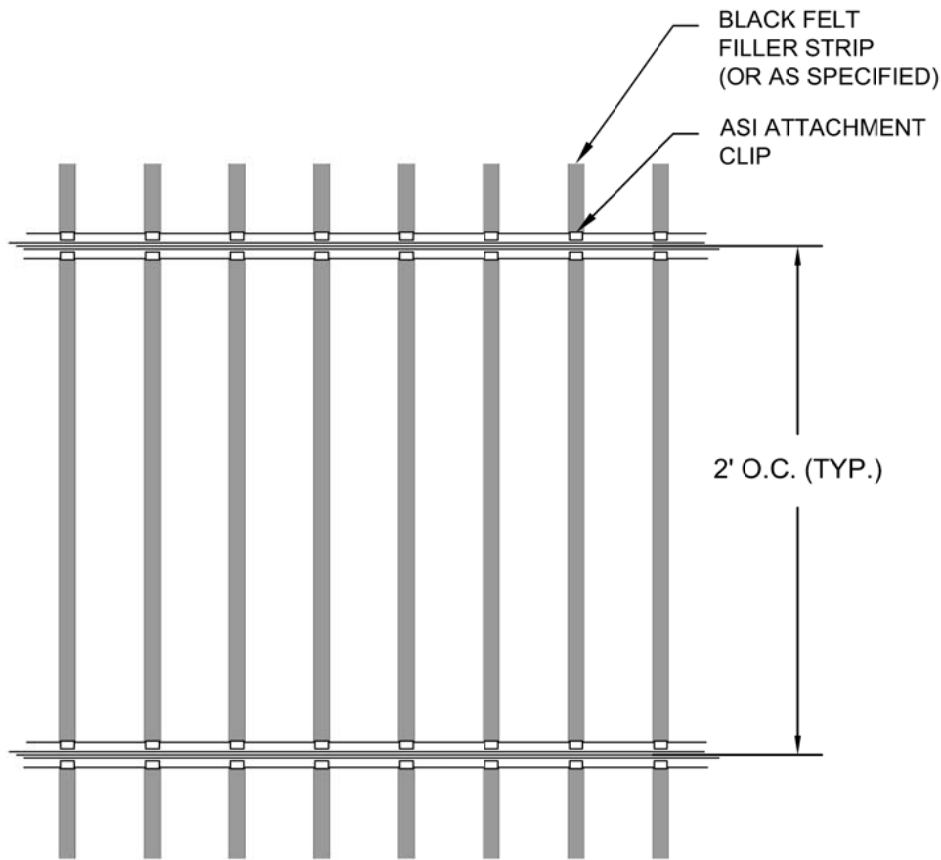
1 PLAN VIEW (TYP.) SCALE: NTS
